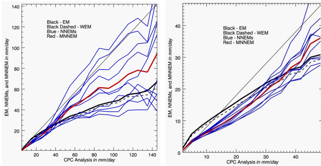
Fig. 4 Binned scatter plots for EM (1) (black solid), WEM (4) (black dashed), ten NNEMs (3) ( NNEM_i , i = 1, \dots, m and m = 10 , all blue), and MNEM (red) that is defined by eq. (5) below. The right panel shows the magnified lower precipitation area.
